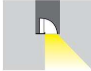
Q-带翻边嵌装 Q-recessed with trim
