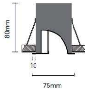
Q-带翻边嵌装 Q-recessed with trim
